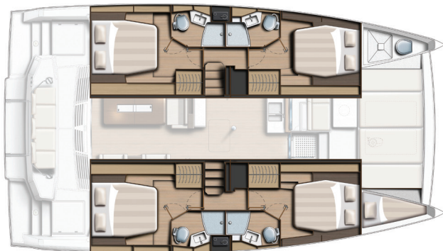
Version 4 cabins - 4 sdb + Skipper (option) / 4 cabins - 4 heads + Skipper (optional)
