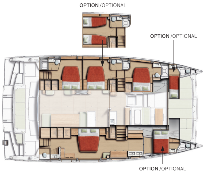
Version 4 cabines (1 master) - 4 sdb + 2 skippers / 4 cabins (1 master) - 4 heads version + 2 skippers
