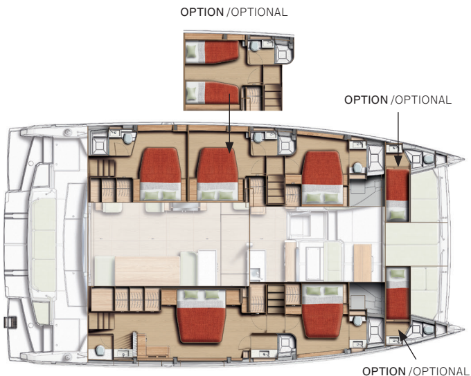
Version 5 cabines (1 master) - 5 sdb + 2 skippers / 5cabins (1 master) - 5 heads + 2 skippers
