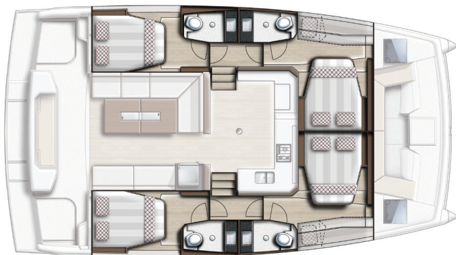
Version 4 cabines - 4 sdb / 4 cabins - 4 heads version
