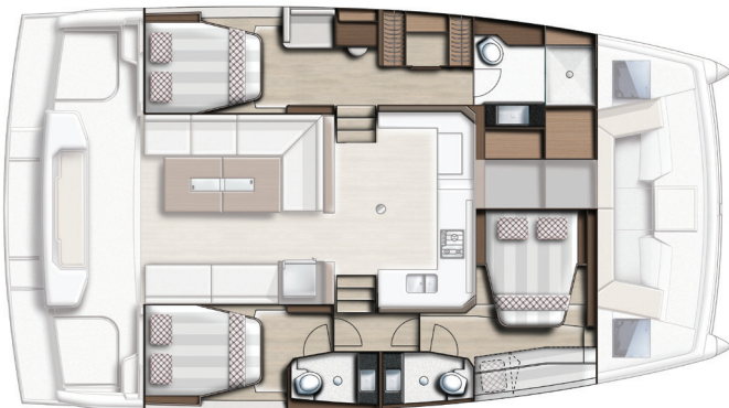
Version 3 cabines - 3 sdb / 3 cabins - 3 heads version
