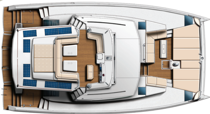
Pont et Flybridge / Deck and Flybridge (optional teak floor)
