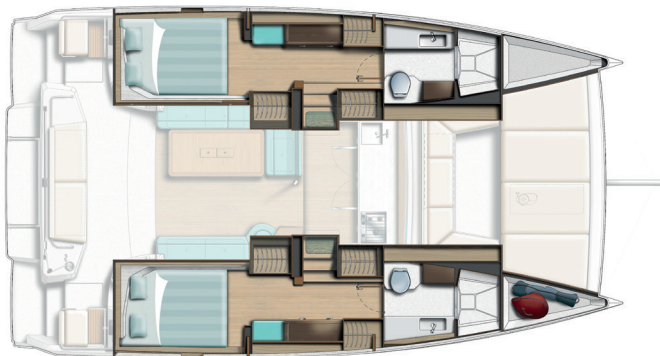
Version 2 cabines - 2 sdb / 2 cabins -2 heads version
