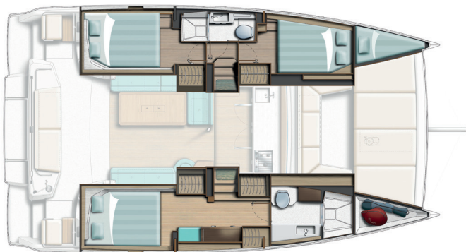
Version 3 cabines - 2 sdb / 3 cabins -2 heads version
