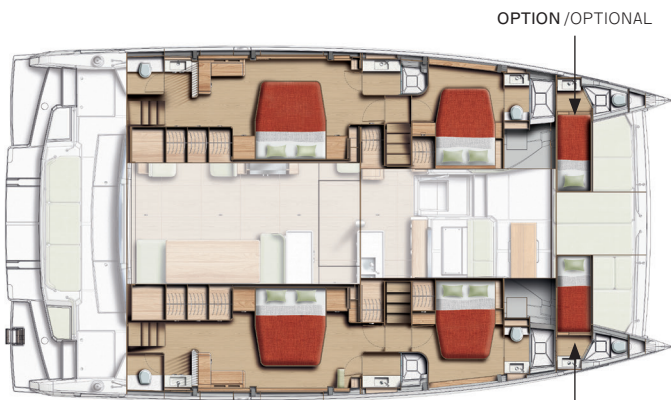
Version 4 cabines (2 masters) - 4 sdb + 2 skippers / 4 cabins (2 masters) - 4 heads + 2 skippers
