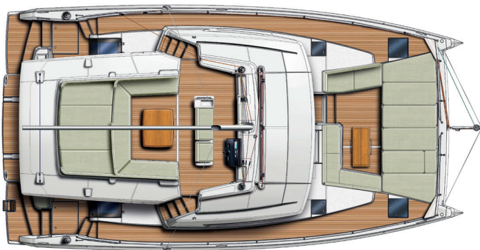
Pont et Flybridge / Deck and Flybridge (optional teak floor)
