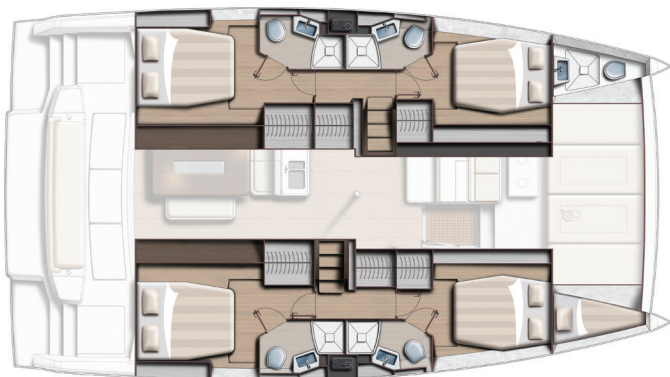
Version 4 cabines - 4 sdb symétriques + 2 singles (option) / 4 cabins - 4 heads symetrical + 2 singles (optional) version
