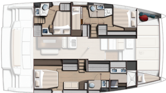
Version Propriétaire 4 cabines - 3 sdb + 1 single (option) / 4 cabins - 3 heads Owner's + 1 single (optional) version
